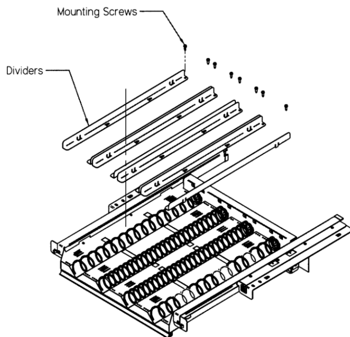
Figure 5.4 1.5" HELIX TRAY
